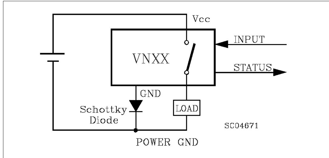
Figure 12. Typical application circuit with a schottky diode for reverse supply protection
